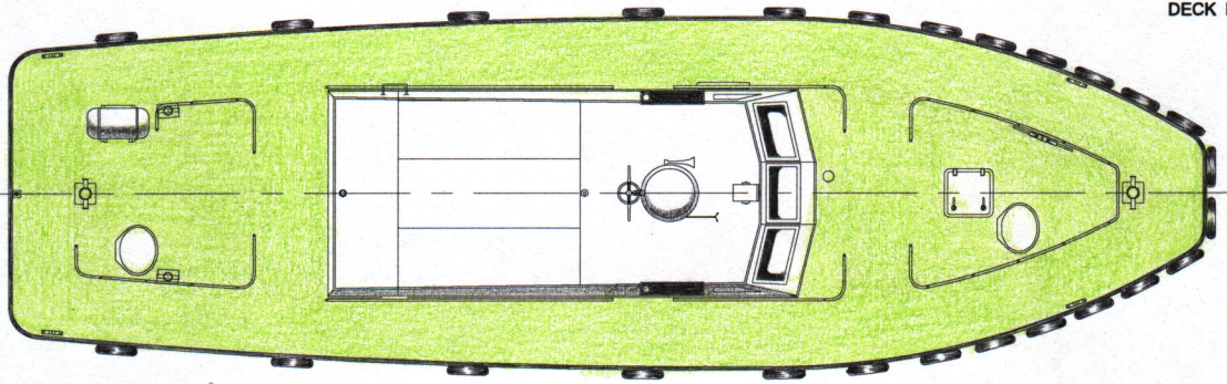
DECK PLAN
