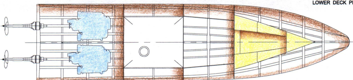
LOWER DECK PLAN
