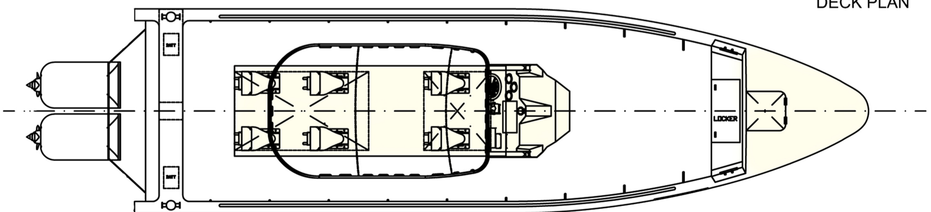
DECK PLAN
