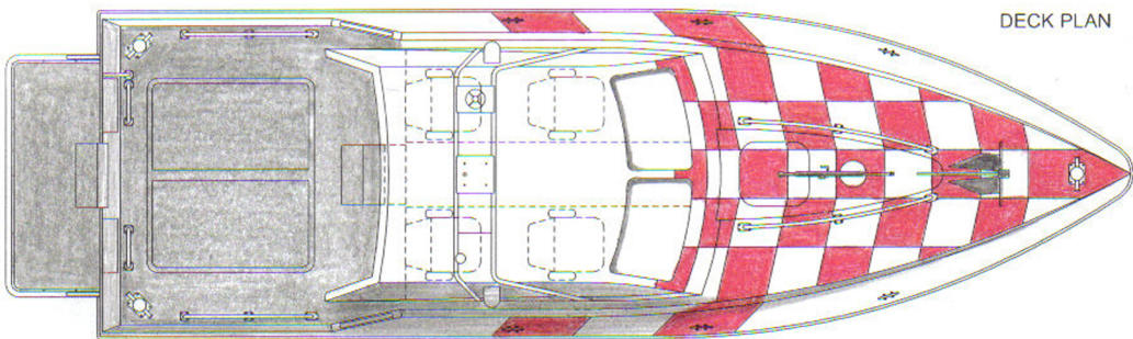
DECK PLAN
