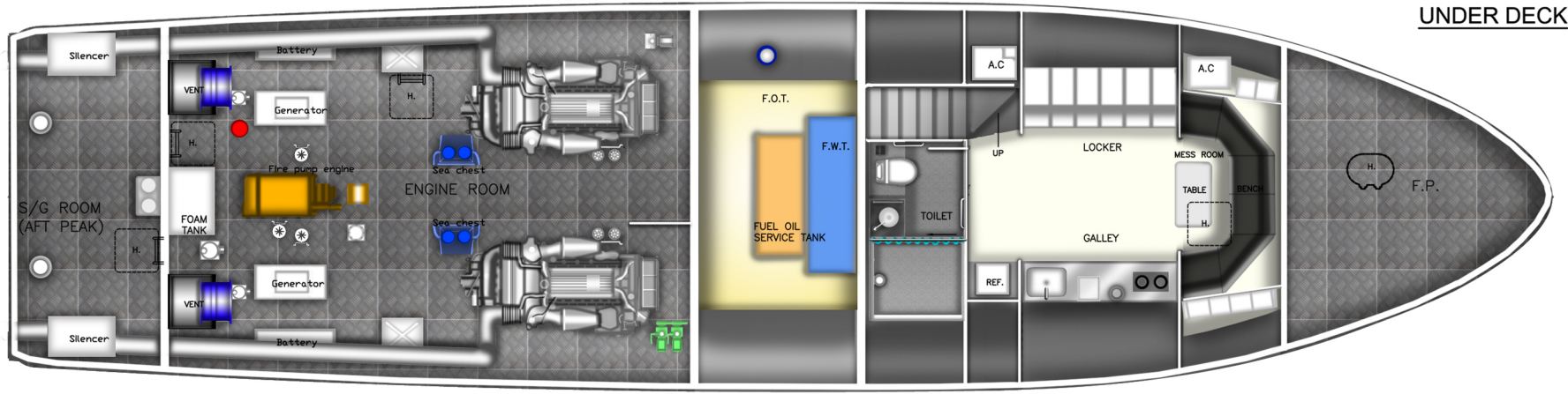
UNDER DECK
