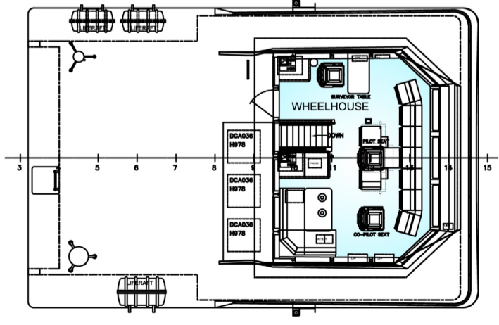
PLAN ON WHEELHOUSE
