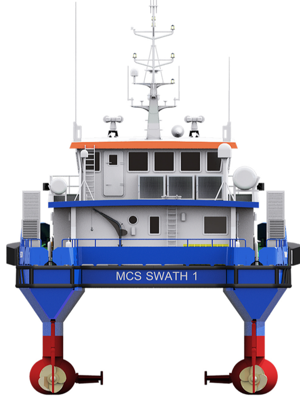
AFT ELEVATION
