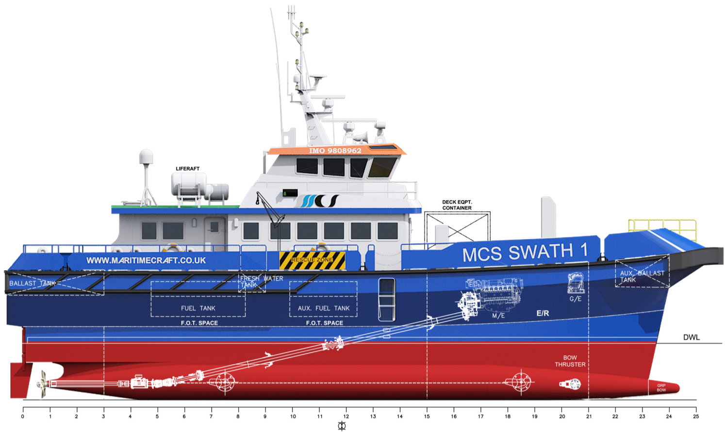
PROFILE VIEW
